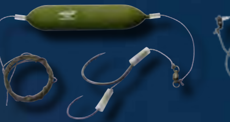
LOBWORM-CALAMARI RIG Rig designed especially for fishing with lobworm bundles or pieces of calamari. Fittings: VMC hook, ball-bearing mounted swivels, abrasion-resistant Catfish Strong line, 30g U-float. The length of the rig can be individually adjusted.
